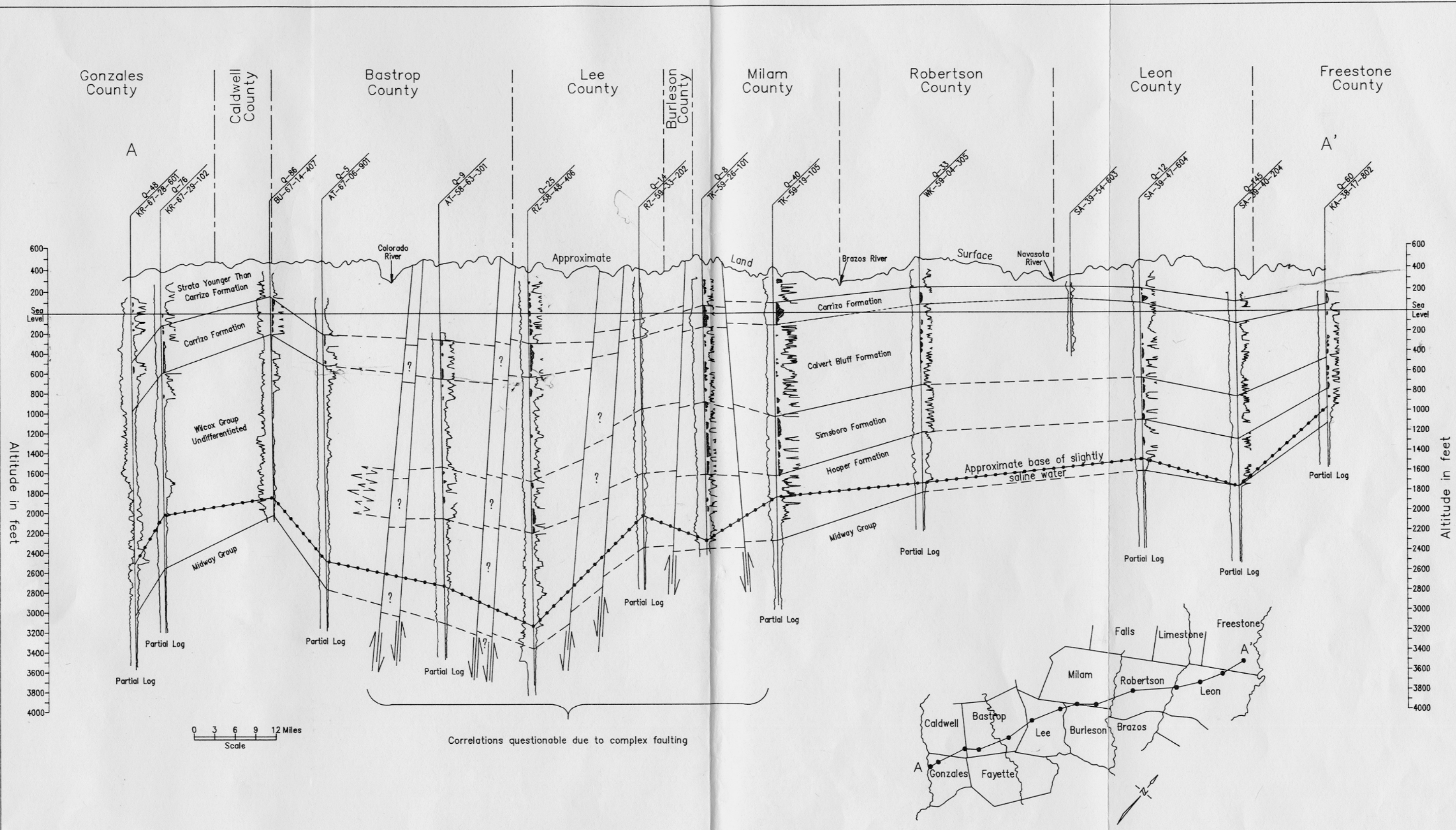
Figure 19 GEOLOGIC SECTION A-A'
